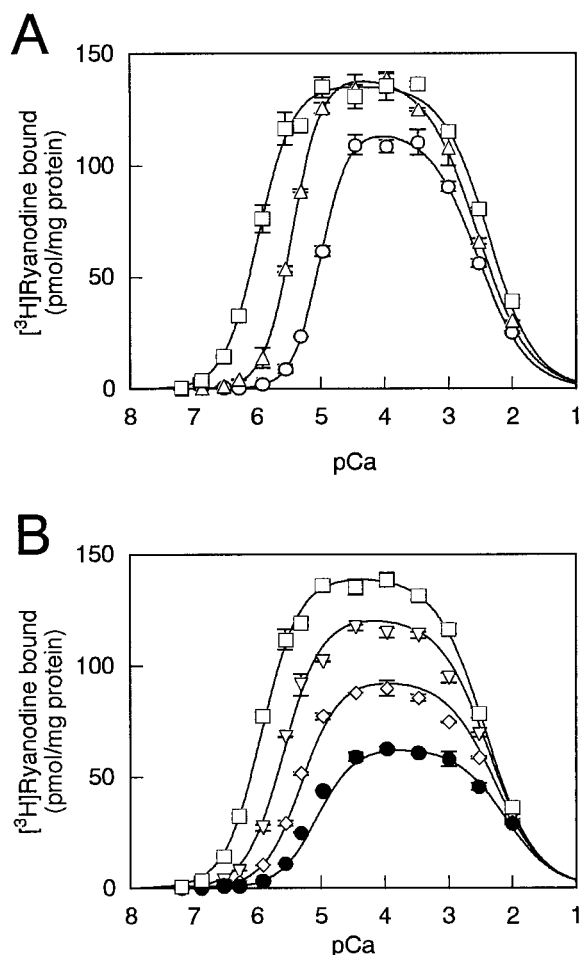
FIGURE 3 (A) Effect of caffeine on the \text{Ca}^{2+} -dependent [\text{H}^3] ryanodine binding to frog RyRs. [\text{H}^3] ryanodine binding to \alpha -RyR was carried out as in Fig. 1 in the presence of 0 ( \circ ), 2 ( \Delta ), and 10 ( \square ) mM caffeine. Data are means \pm half-range of deviations of duplicate determinations. (B) Effect of \text{Mg}^{2+} on the \text{Ca}^{2+} -dependent [\text{H}^3] ryanodine binding in the presence of 10 mM caffeine. [\text{H}^3] ryanodine binding to \alpha -RyR was determined with 0 ( \square ), 0.8 ( \nabla ), 2.5 ( \diamond ), and 5.9 ( \bullet ) mM \text{Mg}^{2+} . Computed curves were drawn using Eq. 1 and the following parameters: B_{\text{max}} = 140.2 pmol/mg protein; K_{\text{A,Ca}} = 1.19 \mu\text{M} ; n_{\text{A,Ca}} = 1.5 ; K_{\text{I,Ca}} = 3.85 mM; n_{\text{I,Ca}} = 1.1 ; K_{\text{A,Mg}} = 379 \mu\text{M} ; n_{\text{A,Mg}} = 1.1 ; K_{\text{I,Mg}} = 4.92 mM; n_{\text{I,Mg}} = 1.1 .
