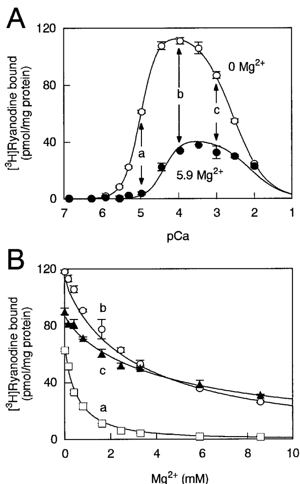
FIGURE 1 Scheme illustrating the procedure for determinations of the affinities for Ca^{2+} and Mg^{2+} of the A- and I-sites of frog RyRs. [^3H] ryanodine binding to the purified \alpha -RyR was carried out as described in Materials and Methods in a reaction medium containing 8.5 nM [^3H] ryanodine, 0.17 M NaCl, 20 mM MOPS/NaOH (pH 6.8), 1% CHAPS, 0.5% phospholipids, 2 mM dithiothreitol, 4 mM AMP, and various free Ca^{2+} and Mg^{2+} . (A) Ca^{2+} dependence of the ryanodine binding in the presence (●) and absence (○) of 5.9 mM Mg^{2+} . Data are means \pm SE ( n = 4 ). (B) Dose-dependent inhibition by Mg^{2+} of [^3H] ryanodine binding at three different Ca^{2+} concentrations (arrows a–c are as indicated in A): 10.7 \mu M (a), 110 \mu M (b), and 1.0 mM (c). Data are means \pm SE ( n = 3 ). Parameters for Ca^{2+} and Mg^{2+} of the A- and I-sites were determined in three consecutive steps. First, the data in the absence of Mg^{2+} (○ in A) were fitted to Eq. 2 to yield the following parameters: B_{max} = 117.4 pmol/mg protein; K_{A,Ca} = 10.1 \mu M ; n_{A,Ca} = 2.0 ; K_{I,Ca} = 2.73 mM; n_{I,Ca} = 1.0 . Second, the dose-dependent inhibition by Mg^{2+} (▲ in B) in the presence of 1 mM Ca^{2+} (arrow c in A), where competition of Mg^{2+} for the A-site is negligible, was fitted to Eq. 3 to obtain K_{I,Mg} (3.16 mM) and n_{I,Mg} (0.9). Third, the data (□ in B) at 10.7 \mu M Ca^{2+} (arrow a in A), where competitive inhibition by Mg^{2+} is prominent, were fitted to Eq. 1 to estimate K_{A,Mg} (396 \mu M ) and n_{A,Mg} (1.1). The validity of the obtained parameters was confirmed by comparing the curve computed according to Eq. 1 with the data (curve b in B) at 110 \mu M Ca^{2+} (arrow b in A). These parameter values were also verified by the curve fit to the Ca^{2+} -dependent [^3H] ryanodine binding in the presence of 5.9 mM Mg^{2+} as shown in A.
