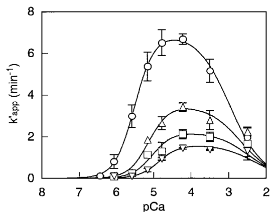
FIGURE 4 Effect of \text{Mg}^{2+} on the \text{Ca}^{2+} dependence of CICR in skinned muscle fibers. Rate constants of the \text{Ca}^{2+} release from SR using six skinned fibers were determined in the CI medium containing 4 mM AMP and various \text{Ca}^{2+} concentrations. Effects of various \text{Mg}^{2+} concentrations were examined: 0 ( \circ ), 0.4 ( \Delta ), 0.8 ( \square ), or 1.6 mM ( \nabla ) \text{Mg}^{2+} . The results, corrected for as described in Materials and Methods, are plotted. pH was adjusted to 7.0 for these experiments. Parameters determined according to the procedure described in Fig. 1 were k_{\text{max}} = 7.0 \text{min}^{-1} , K_{\text{A,Ca}} = 3.2 \mu\text{M} , n_{\text{A,Ca}} = 1.6 , K_{\text{I,Ca}} = 1.1 mM, K_{\text{I,Mg}} = 0.42 mM, K_{\text{A,Mg}} = 0.15 mM. The drawn lines are curves calculated for indicated \text{Mg}^{2+} concentrations, using these parameters. n_{\text{I,Ca}} , n_{\text{A,Mg}} , and n_{\text{I,Mg}} were fixed at 1.0 in these simulations.
