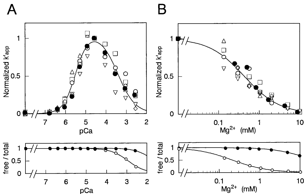
FIGURE 5 Comparison of effects of AMP and AMPPCP on \text{Ca}^{2+} and \text{Mg}^{2+} dependences of CICR in skinned fibers. (A) \text{Ca}^{2+} dependence in the absence of \text{Mg}^{2+} . The top panel shows \text{Ca}^{2+} dependence of the relative k'_{app} , which was normalized with the value at pCa 4.5. CICR was determined in the Ms medium containing 4 mM AMP (●) or 0.2 mM AMPPCP (○, □, △, ▽, ◇). Different symbols indicate different preparations. The bottom panel indicates the calculated fractions of the free form to total AMP (●) or AMPPCP (○). AMP is mostly in the free form, whereas the complexed form of AMPPCP makes up a considerable fraction of the total. The solid line in the top panel was drawn based on data with 0.2 mM AMPPCP according to Eq. 2, where the parameters were K_{A,Ca} = 3.9 \mu\text{M} , n_{A,Ca} = 1.4 , K_{I,Ca} = 0.43 \text{ mM} , and n_{I,Ca} = 1 . (B) \text{Mg}^{2+} -dependent inhibition in the presence of 90 \mu\text{M} \text{Ca}^{2+} is shown in the top panel, and the calculated ratio of free to total nucleotide is shown in the bottom panel. The results were normalized with those in the absence of \text{Mg}^{2+} . The drawn line shows the curve of Eq. 3 best fit to data with 0.2 mM AMPPCP, where parameters were K_{I,Mg} = 0.36 \text{ mM} and n_{I,Mg} = 1.0 , in addition to those determined in A. Note that CICR activities in the presence of AMP and AMPPCP showed very similar \text{Ca}^{2+} (A) and \text{Mg}^{2+} dependences (B), although their ratio of the free form to total nucleotides was very different in the presence of high concentrations of \text{Ca}^{2+} and \text{Mg}^{2+} .
