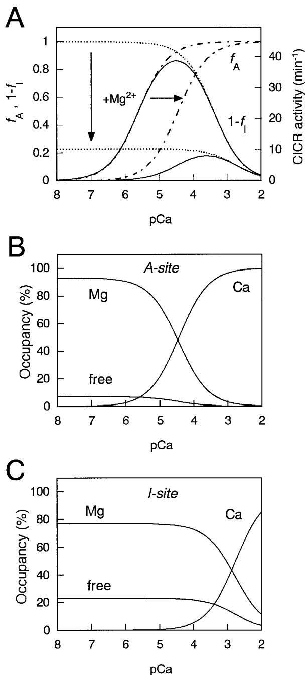
FIGURE 8 Simulations of effects of \text{Mg}^{2+} on the CICR activity in situ and analysis of the occupancy by divalent cations of the A- and I-sites. (A) The fractions of \text{Ca}^{2+} -occupied A-site ( f_A ) and vacant I-site ( 1-f_I ) and the anticipated CICR activity ( k = k_{\text{max}} \times f_A \times (1-f_I) ) were calculated in the presence or absence of 1 mM \text{Mg}^{2+} . f_A (---), 1-f_I (.....), and k (—) were calculated as a function of free \text{Ca}^{2+} , using the following parameters, which are assumed to be those for the \text{Ca}^{2+} release channel of SR in situ: k_{\text{max}} = 45 \text{ min}^{-1} ; K_{A,\text{Ca}} = 2.5 \text{ }\mu\text{M} ; n_{A,\text{Ca}} = 1 ; K_{I,\text{Ca}} = 0.4 \text{ mM} ; n_{I,\text{Ca}} = 1 ; K_{A,\text{Mg}} = 75 \text{ }\mu\text{M} ; n_{A,\text{Mg}} = 1 ; K_{I,\text{Mg}} = 0.3 \text{ mM} ; n_{I,\text{Mg}} = 1 . We assumed n_{A,\text{Ca}} to be 1 in the presence of 4 mM AMPPCP, based on the finding that n_{A,\text{Ca}} values decreased with an increase in AMPPCP concentration (from 1.4 at 0.2 mM to 1.2 at 1 mM; see Table 3). \text{Mg}^{2+} (1 mM) shifts curve f_A rightward along the abscissa to decrease the apparent \text{Ca}^{2+} sensitivity and reduces (1-f_I) throughout all \text{Ca}^{2+} concentrations, resulting in the
